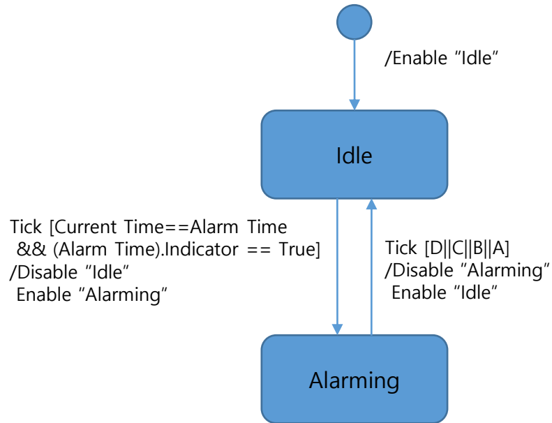
Alarm Controller
